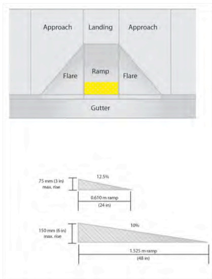
Curb ramp components, and alternate ramp slopes (Credit: Michele Weisbart)
